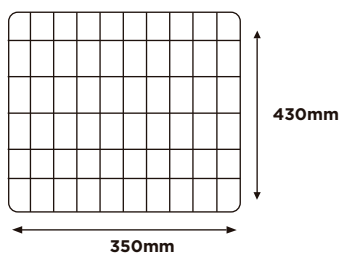
PANEL SOLAR
