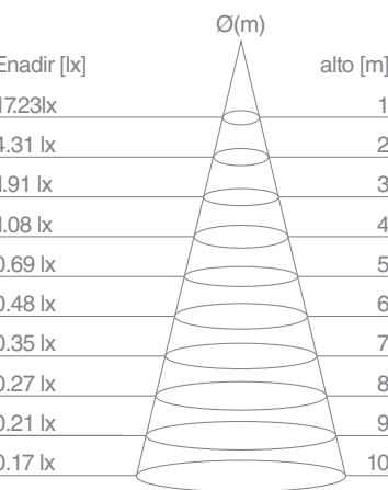
Vintage ST19 8W Dimeable
