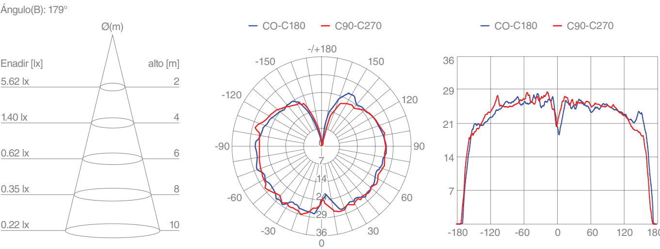
Vintage ST19 5W
