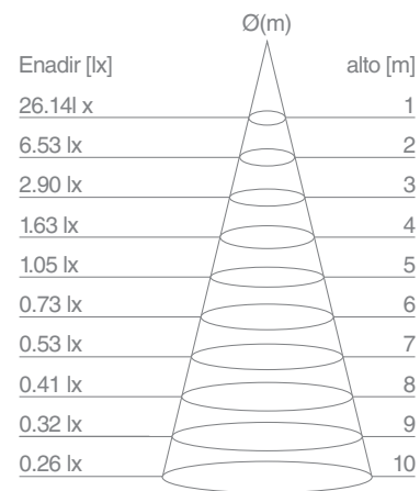
Globo G125 8W Dimeable
