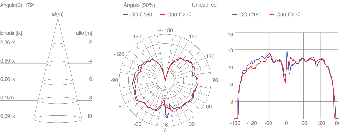
Vintage ST19 5W
